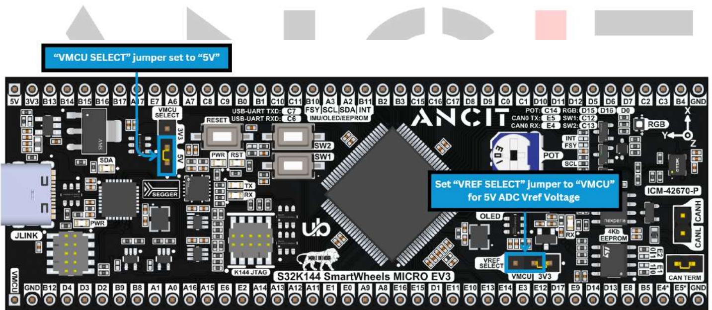
Fig 8 : ADC VRef set to 5V
