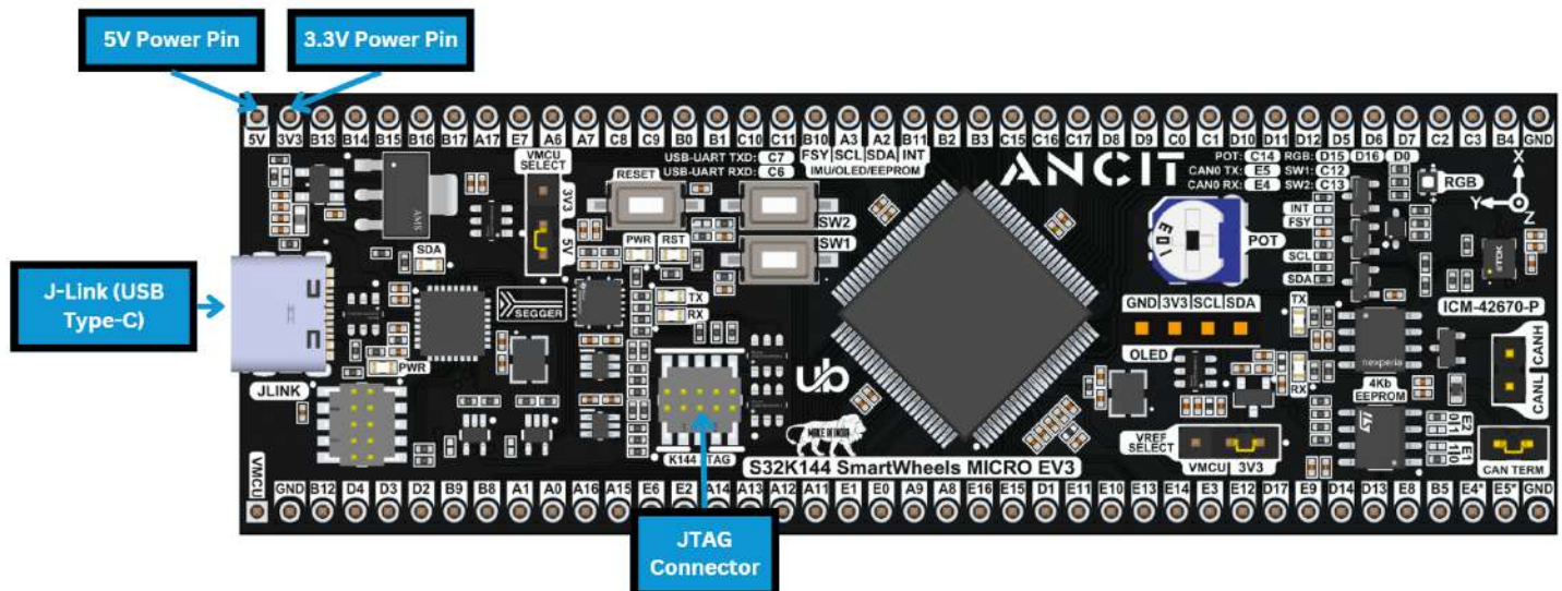
Fig 1 : Power Inputs for SmartWheels EV3
