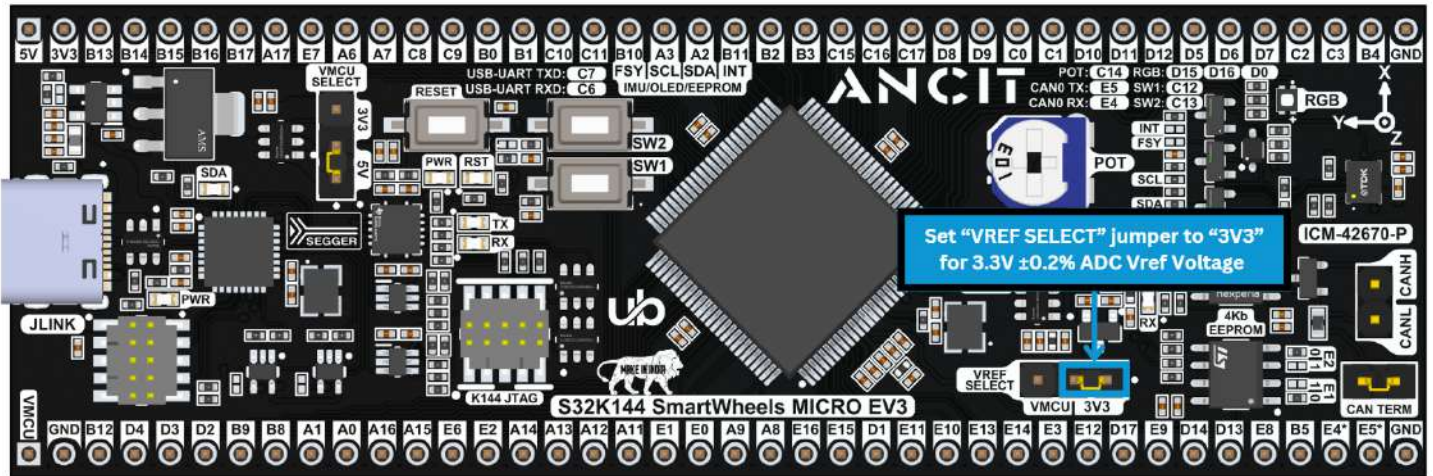
Fig 7 : ADC VRef set to 3.3V ±0.2% Voltage Reference
