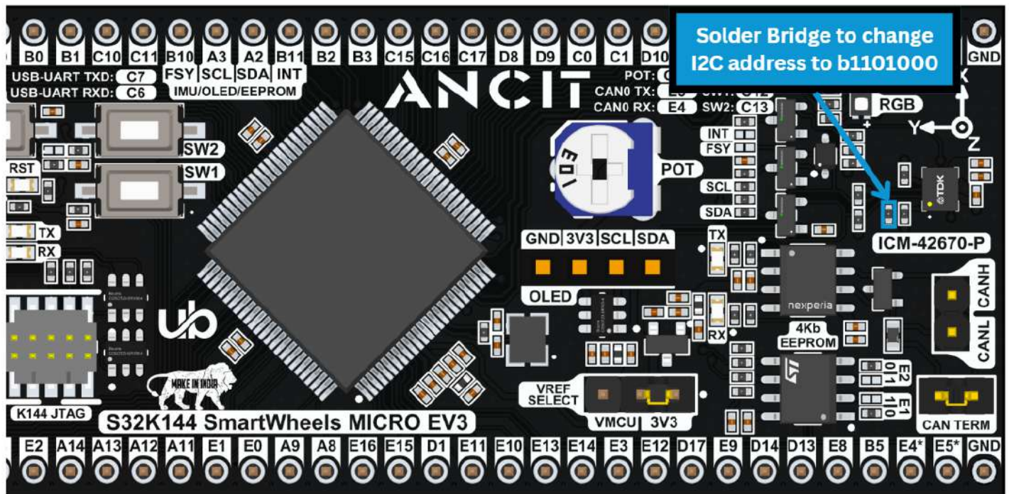
Fig 16 : I2C Address Selection Jumper Resistors
