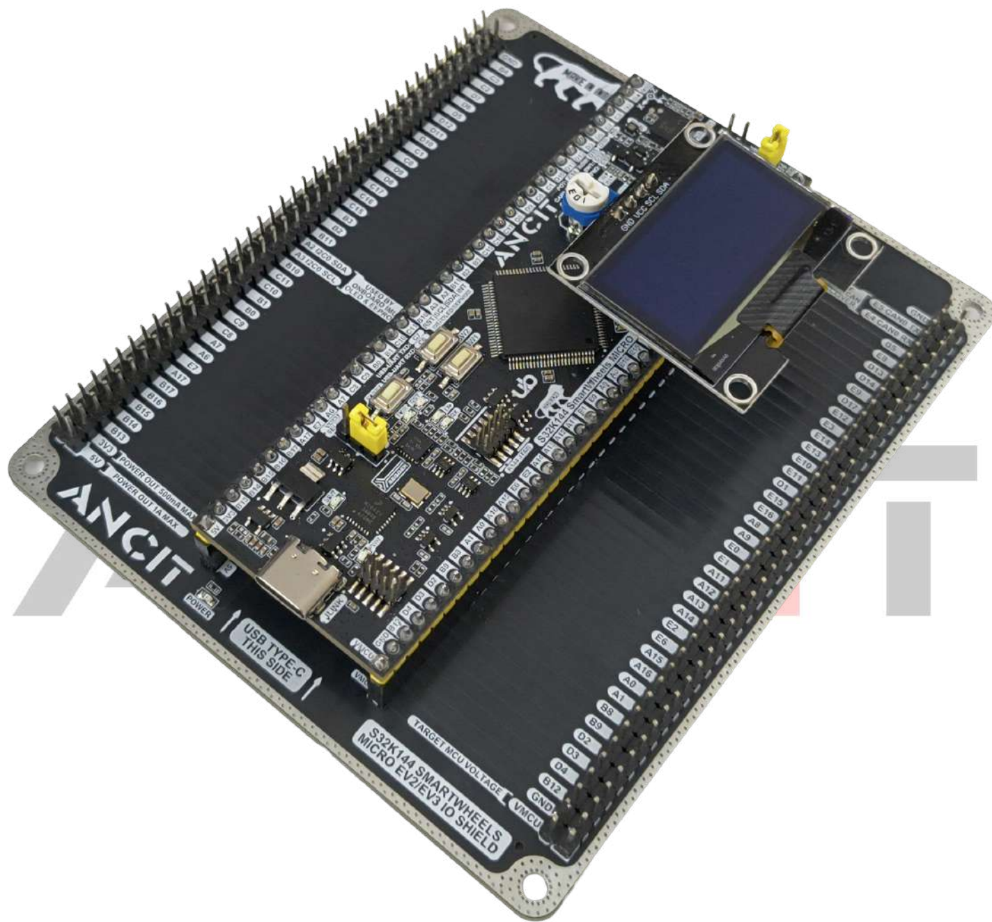
S32K144 SmartWheels Micro EV3 with OLED Display + SmartWheels IO Shield
