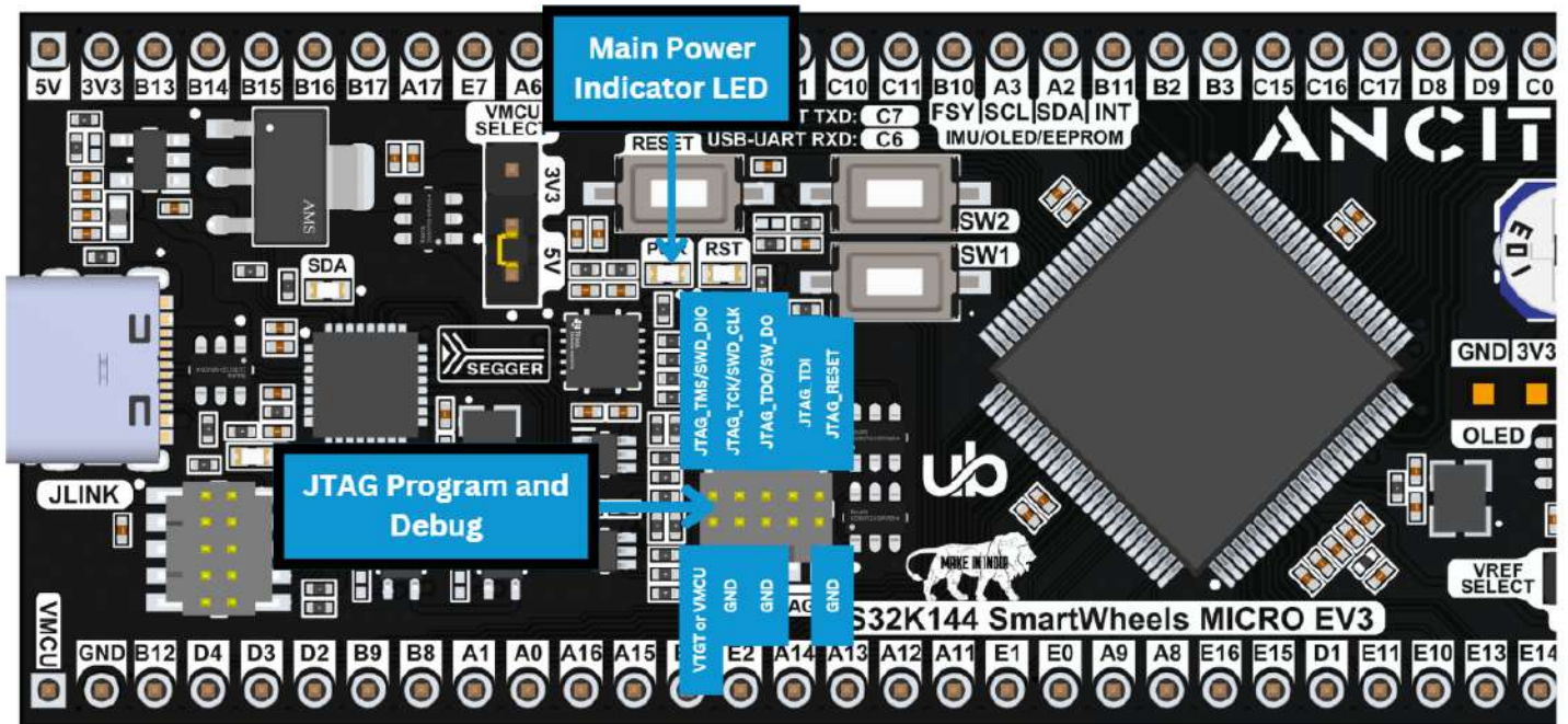
Fig 11 : JTAG connector on SmartWheels EV3
