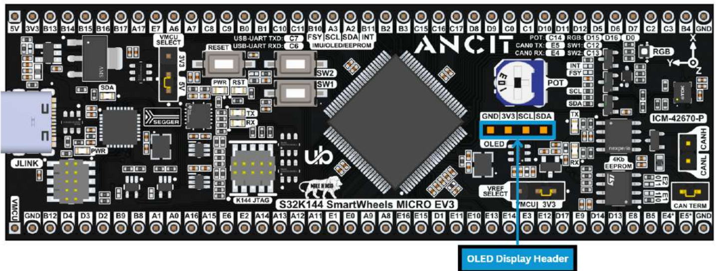
Fig 19 : Onboard headers for OLED display
