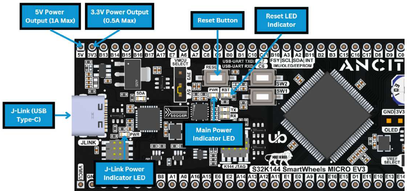
Fig 9 : J-Link Jumper Settings and Indicator LEDs
