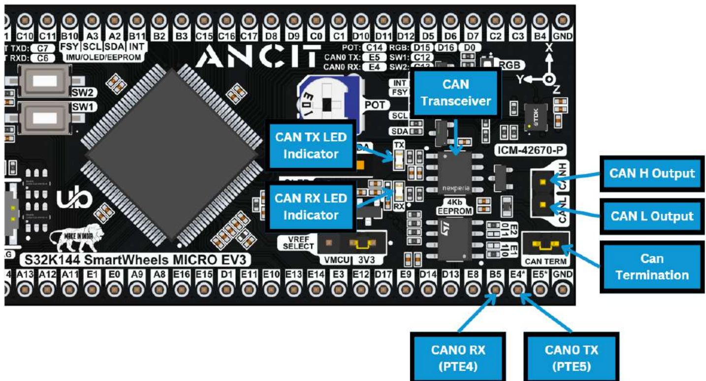
Fig 12 : CAN output, CAN Termination and Data Indicators LEDs
